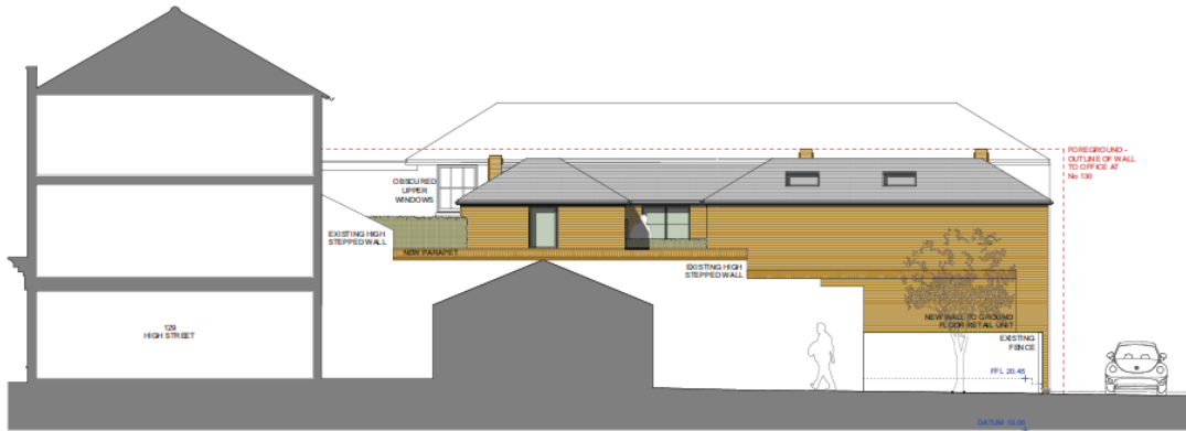
NORTH ELEVATION / SECTION B-B
