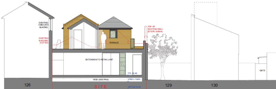
SIDE TERRACE ELEVATION / SECTION F-F
